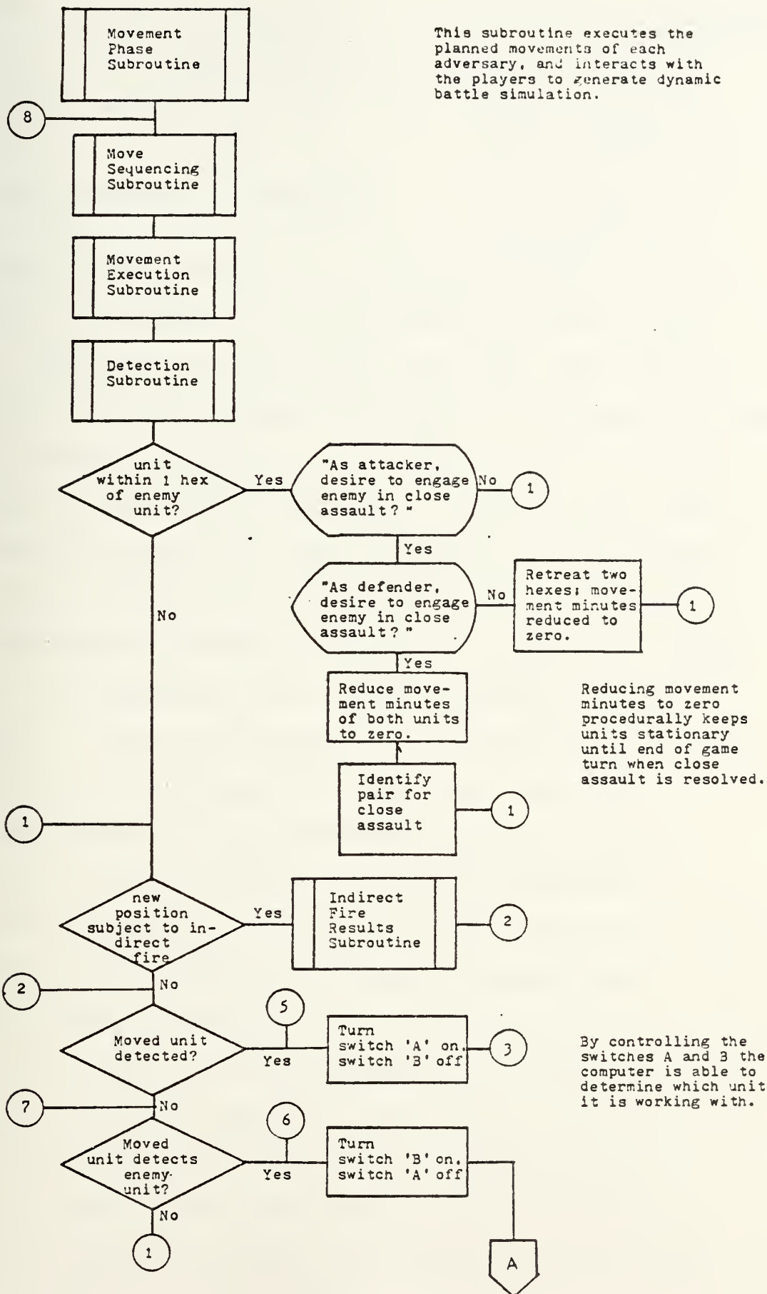
FIGURE VII.1 FLOWCHART OF MOVEMENT PHASE SUBROUTINE
